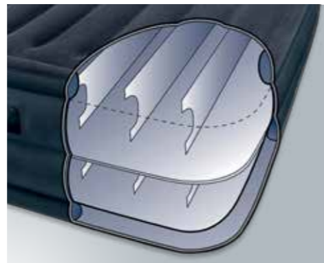
Double-Layered Wave Beam Construction
