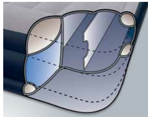
Deluxe Pillow Rest Construction
