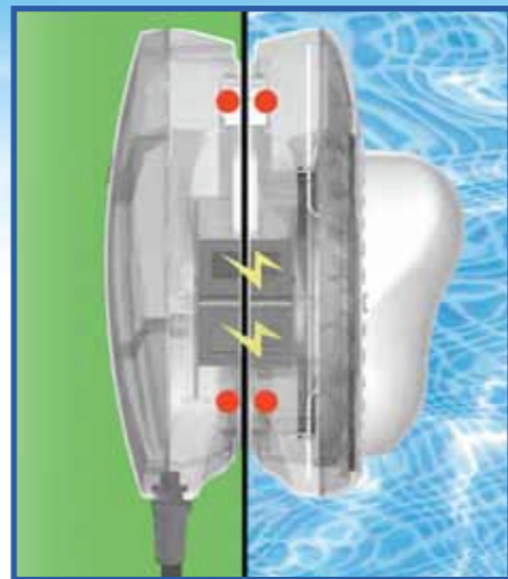
The outside part transmits power safely and wirelessly to inside the underwater LED where the magnetic technology holds the two parts together.
